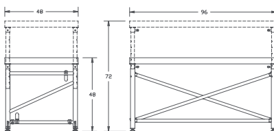
All-Terrain Style SC9600 Bridge Support System
