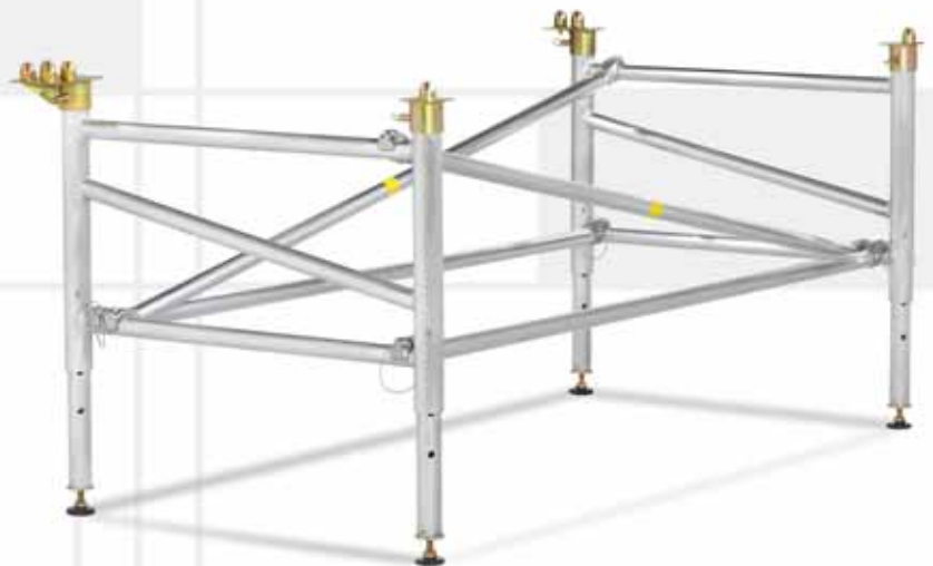
SC9600 Bridge Support System without Platform
